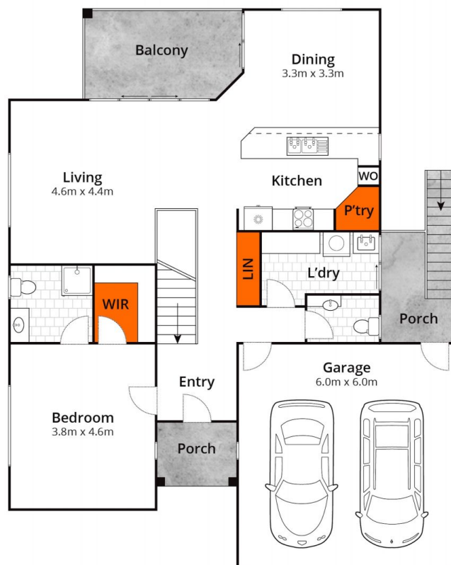
Upper Floor
