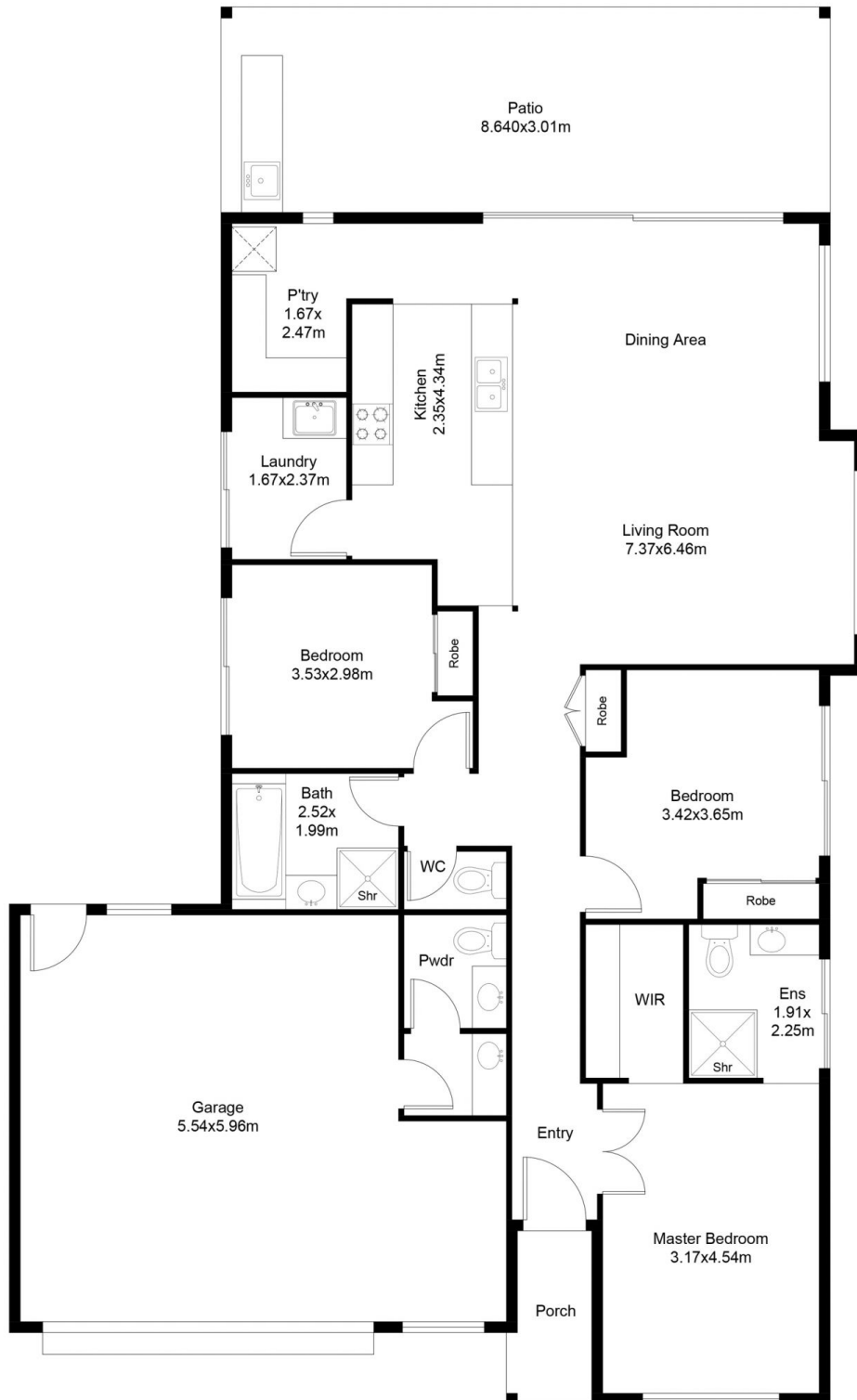
FLOOR PLAN
